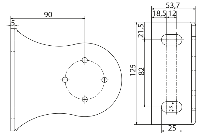
Wall ceiling brackets
