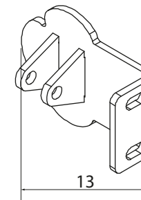
Arm lateral support
