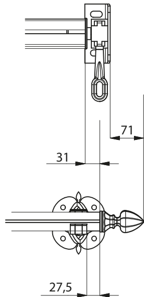
Lateral encumbrances of the awning
